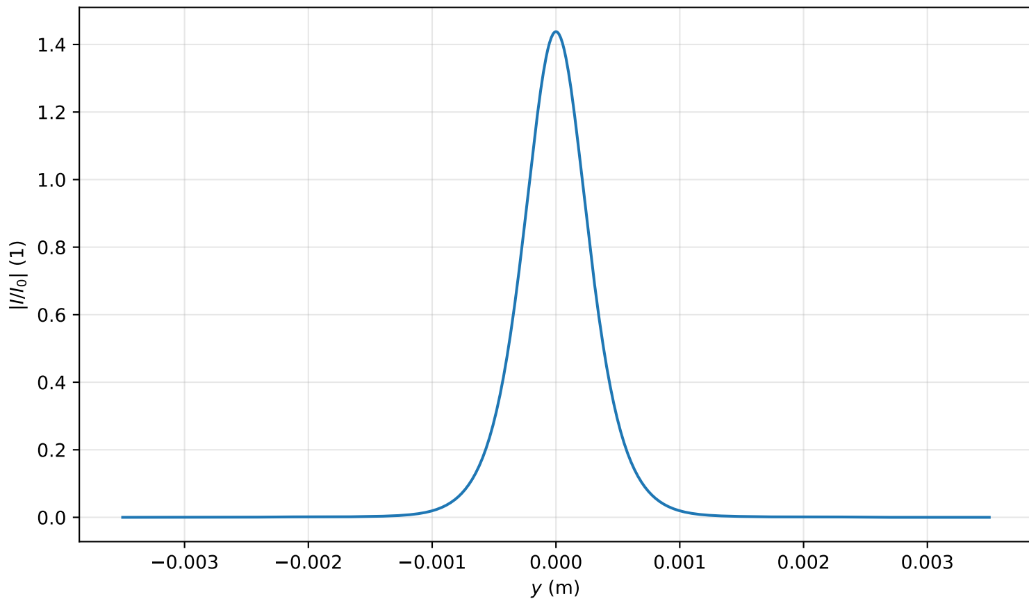
Intensity profile I(x=0, y, z=3.821)/I_0 , \text{Pin}=0.9\text{Pcr} , artificial time
